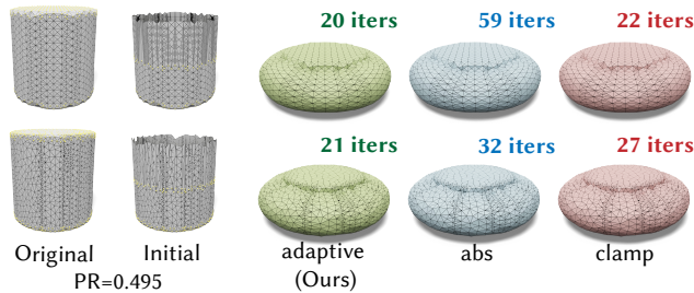
Fig. 13. Our method is robust to different tetrahedralizations. Here we tetrahedralize the same cylinder to two different tetrahedral meshes. The meshes on the top and bottom row have 6.1k and 6.6k vertices, respectively. In both settings, our method outperforms existing strategies.
