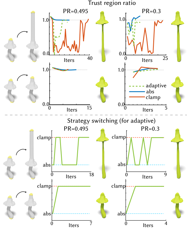
Fig. 6. We visualize the trust-region ratio \rho (for all strategies) and strategy switching trend (for adaptive) during the optimization under different deformations and Poisson’s ratios. While the trust region ratio can change drastically in the early stage of optimization for the highly nonconvex energy landscape—e.g., large deformation and high Poisson’s ratio, it usually approaches 1 near convergence. Thus the adaptive strategy often starts from abs strategy for the first few iterations, alternates between abs and clamp during the optimization, and falls back to clamp near convergence. On the contrary, solely using the abs strategy may excessively damp the descent direction when the quadratic approximation is still acceptable (e.g., small PR or volume change) or later becomes good (e.g., near convergence).
