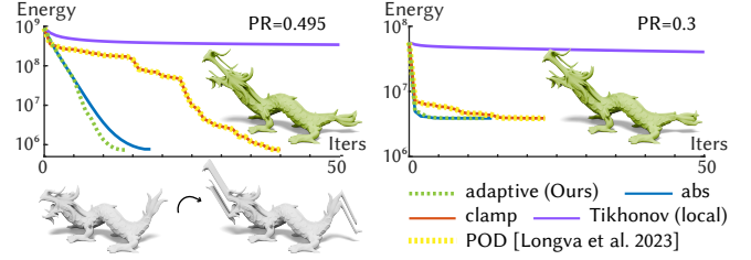
Fig. 9. We compare the energy convergence curve in our approach, the Projection-On-Demand (POD) [Longva et al. 2023] and per-element Tikhonov regularization. We also note that, separate from the optimization convergence performance, POD may require additional Cholesky decompositions to check the positive definiteness of the Hessian.
