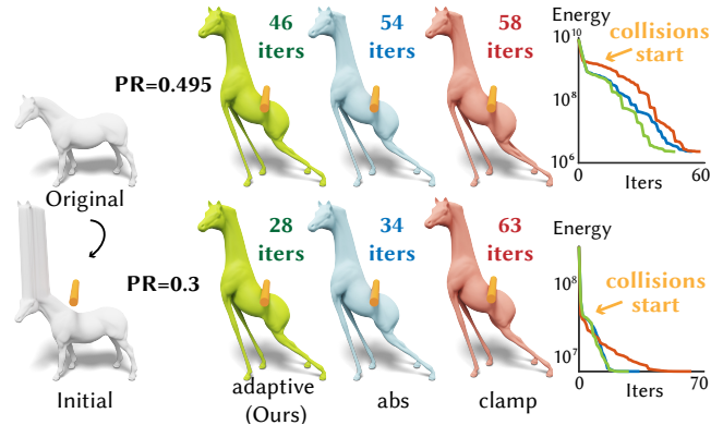
Fig. 11. We perform a collision experiment using Incremental Potential Contact (IPC) [Li et al. 2020] by placing a cylinder (orange) above the back of a horse. Note that IPC’s intersection-aware line search dominates convergence and step size after collisions happen. Extending our framework to accelerate the convergence of barrier functions could be an interesting future direction.
