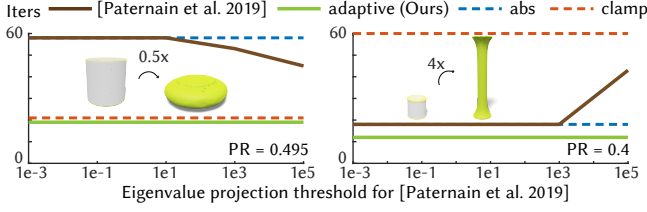
Fig. 7. We compare our method to a per-element version of the eigenvalue projection scheme in [Paternain et al. 2019]. Due to the large variation across local elements’ eigenvalue magnitudes (under different deformations and Poisson’s ratios), it is unclear how to set an eigenvalue projection threshold for [Paternain et al. 2019]. Here, we sweep through a range of threshold values (x-axis) and plot the needed number of iterations in each setting. Our method is consistently more efficient.
