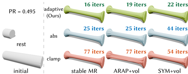
Fig. 10. Our adaptive strategy generalizes across different Neo-Hookean variants. Here in the last three columns, we experiment with different strain energies, including Mooney-Rivlin, ARAP, and Symmetric Dirichlet energy, each augmented with a volume-preservation term (J - 1)^2 .
