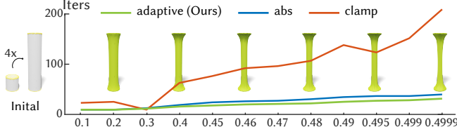
Fig. 5. Here, the cylinder is stretched to 4\times of its rest length. We increase the cylinder’s Poisson’s ratio (x-axis) and test the number of iterations (y-axis) needed for convergence in our method and the comparing methods. Across the entire range of Poisson’s ratios, our method consistently outperforms others.
