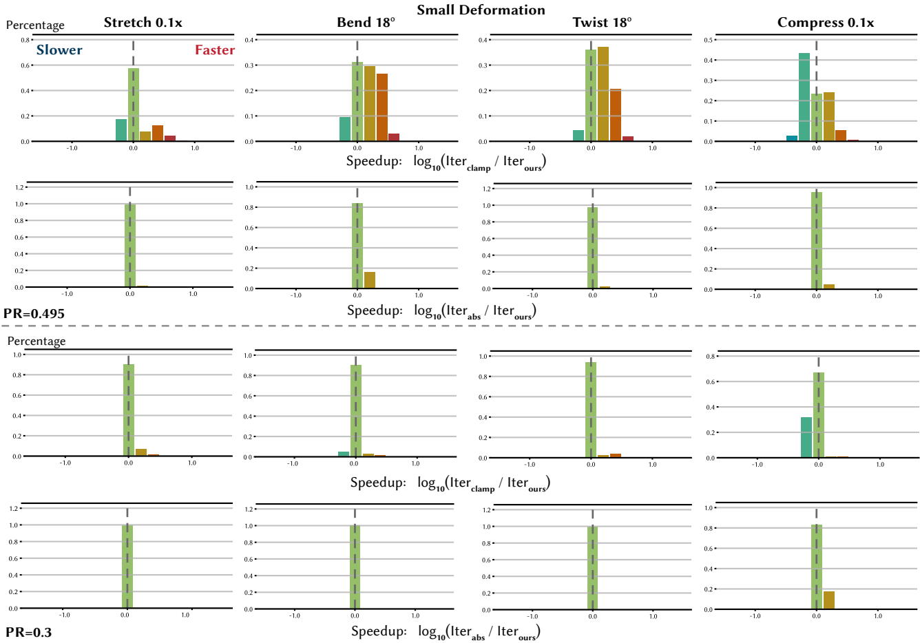
Fig. 14. Histogram of the speedup of our adaptive method in settings similar to Fig. 12 but with much smaller deformations. Even in these simple scenarios, our method outperforms eigenvalue clamping under a large Poisson’s ratio, and performs comparably in other cases.
