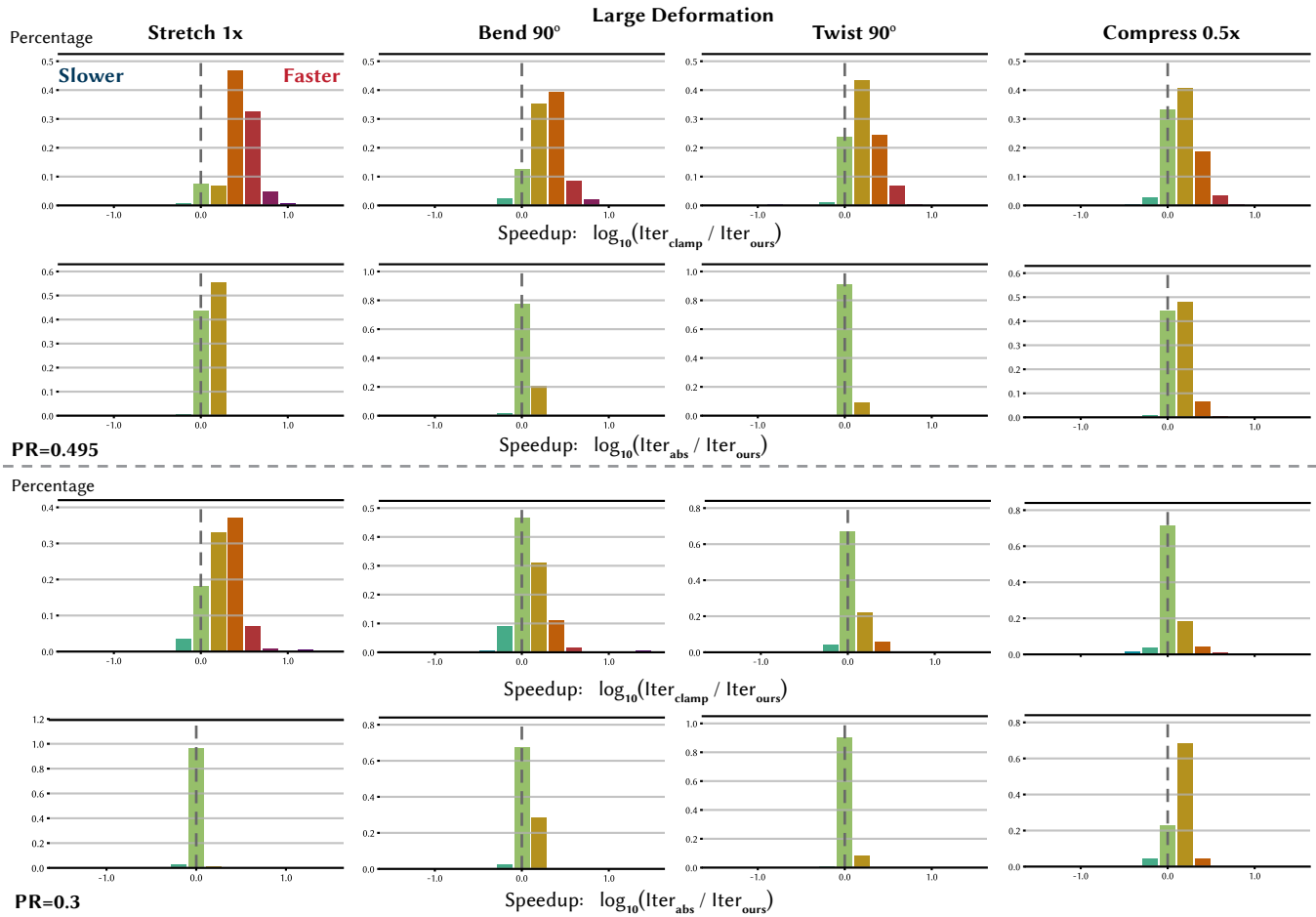
Fig. 12. Histogram of the speedup of our adaptive method over the absolute eigenvalue projection [Chen et al. 2024] and eigenvalue clamping [Teran et al. 2005] on TetWild Thing10k dataset. Here, we test with a diverse set of large deformations (shown in each column). First row: speedups over eigenvalue clamping with a Poisson’s ratio 0.495. Second row: speedups over absolute eigenvalue projection with a Poisson’s ratio 0.495. Third row: speedups over eigenvalue clamping with a Poisson’s ratio 0.3. Fourth row: speedups over absolute eigenvalue projection with a Poisson’s ratio 0.3.
