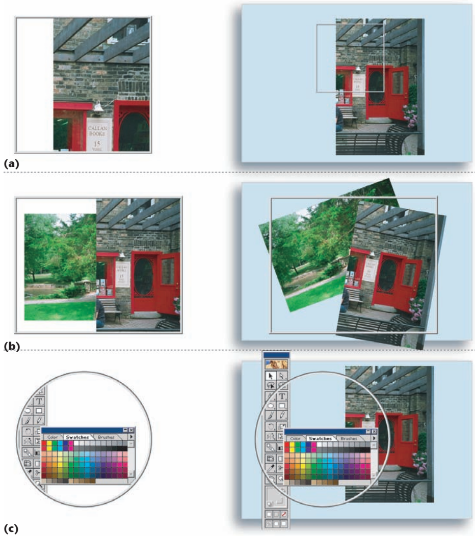
2 Canvas portal shape and attribute example. The left column shows the portal areas of the canvas portals; the right shows the remote focal areas on the displays. (a) Rectangular canvas portal with scale attribute modified to act as a zoom lens to the focal area. (b) Rectangular canvas portal with modified time attribute displaying a previous state of the focal area's content. (c) Circular canvas portal with semantic attribute modified to show only user interface elements, creating a tool palette.
