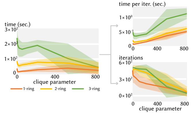
Fig. 25. We show the change of the total ADMM runtime, the ADMM runtime per iteration and the number of iterations with respect to clique parameters when coarsening a number of meshes to 800 vertices. Here the lines denote the average and the color regions denote the standard deviation.
