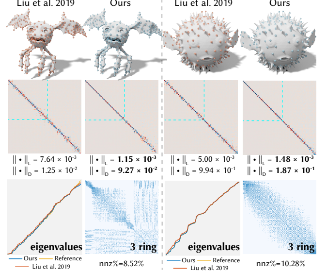
Fig. 8. For applications that desire to preserve low frequencies, our weighted formulation can focus on preserving the first few eigenvectors and eigenvalues (shown in increasing order). Our weighted formulation achieves better results comparing to [Liu et al. 2019] under the same sparsity pattern when coarsening the shapes from 8,000 (left) and 28,000 (right) vertices to 400, respectively. Here we show the Laplacian commutativity norm and Orthonormality norm based on the functional map of the first 50 eigenvectors (inside the dashed lines).
