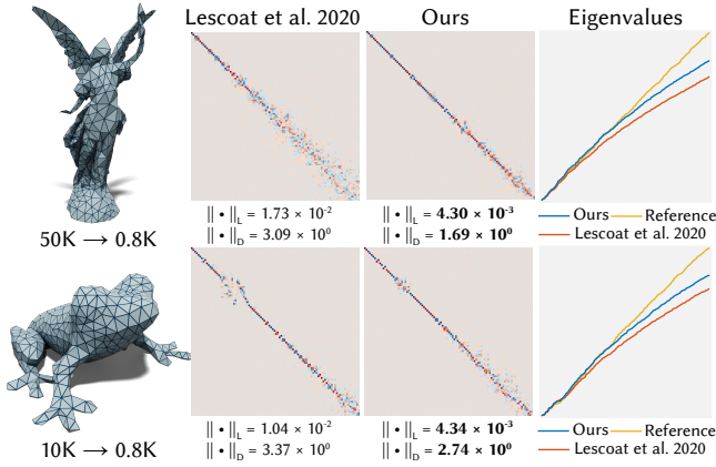
Fig. 17. When the coarsening is aggressive, our method can still postprocess the results of [Lescoat et al. 2020] to improve the quality of spectral preservation.
