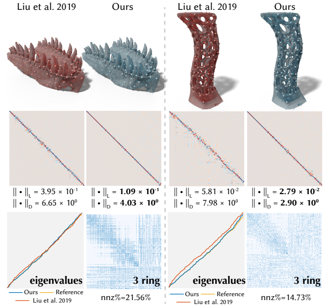
Fig. 9. As degrees of freedom increase for volumetric Laplacian, our method is still able to maintain the spectral properties of the tetrahedral meshes (from 32,000 and 27,000 vertices to 400 respectively) using the same sparsity as [Liu et al. 2019]. Here the eigenvalues are shown in increasing order.
