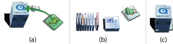
Figure 9. Drag'n'Cross technique for precise insertion. (a) User drags document and crosses Leafer widget, pen path shown by green arrow. (b) Scrub to specify insertion point. (c) Pen is released and document inserted
