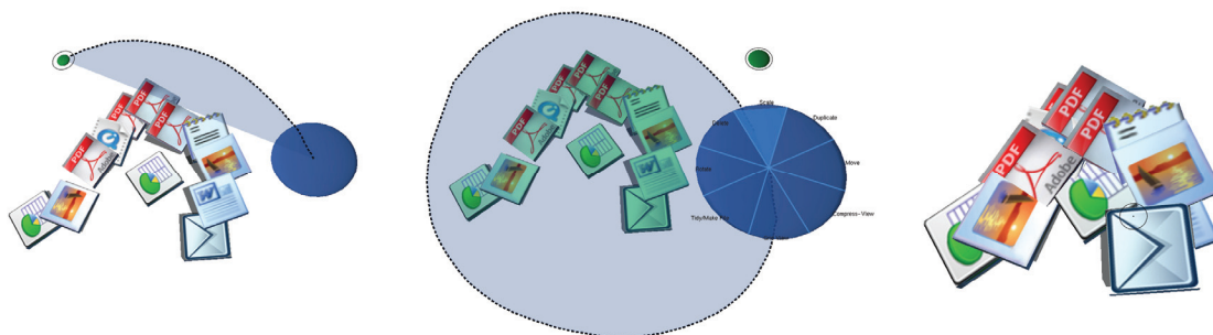
Figure 3. LassoMenu. (left) Lasso selection phase. (center) Lasso completed, pen reaches blue circle and enters control menu. Resize command selected. (right) Remainder of pen movement adjusts resize parameter.
