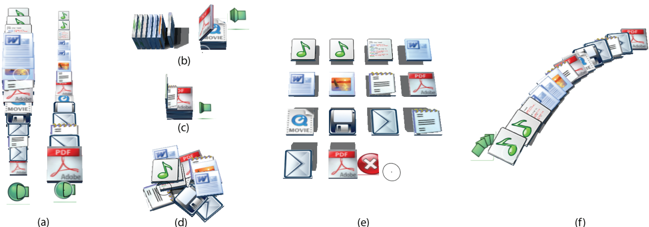
Figure 6. Pile browsing layouts triggered by widgets. (a) Fisheye. (b) Leafing through like pages of a book. (c) Compression-Browsing higher items to view items below. (d) Interpolating between Messy and Tidy positions. (e) Grid browse, locked down for further manipulation with PressureLock. (f) Fan out on user drawn path.
