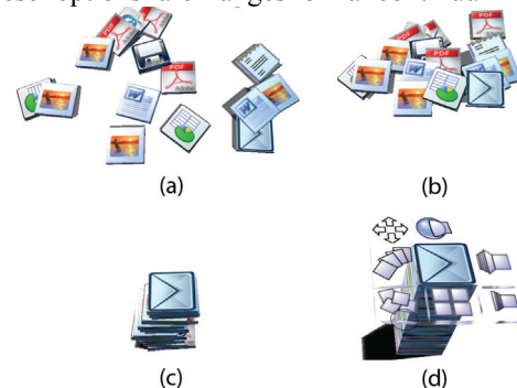
Figure 5. (a) Casually laid out documents. (b) Tidied unpiled documents. (c) Documents made into a Messy Pile. (d) A Tidy Pile with widgets revealed. Widgets in clockwise order from center-top: Fisheye, Leafer, Compression-Browse, Grid, Messy/Tidy, Fan out, Move.
