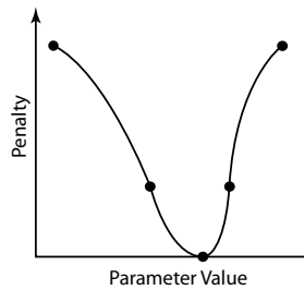
Figure 5: The penalty function consists of desired point and four cubic Hermite curve segments that increase the penalty as the parameter moves away from the desired point.
