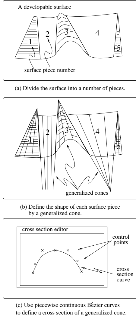
Figure 3: Dividing a developable surface into patches and defining each surface patch by a generalized cone.
