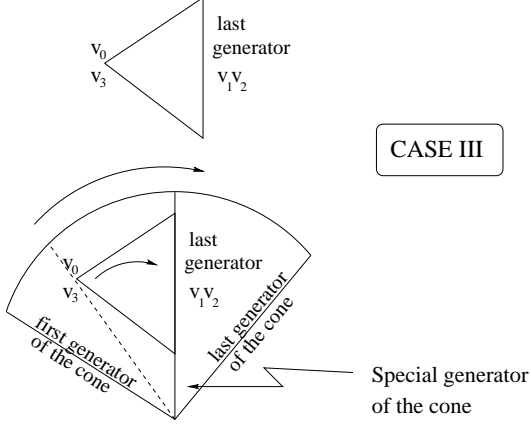
Figure 10: Surface patch type: Case III.
