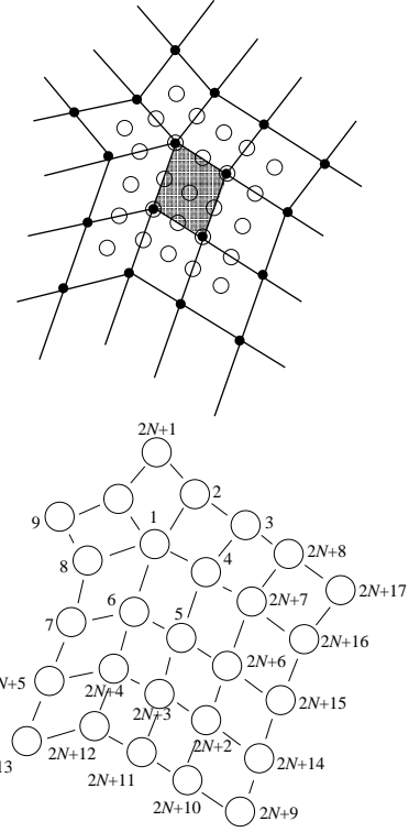
Figure 5: Addition of new vertices by applying the Catmull-Clark subdivision rule to the vertices in Figure 3.
