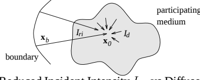
Fig. 1. Reduced Incident Intensity I_{ri} vs Diffuse Intensity I_d
