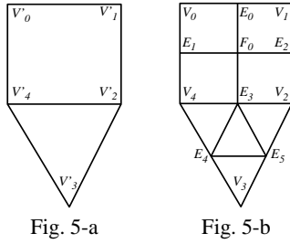
Figure 5: Subdivision of quadrilaterals and triangles. Each subdivision produces V , E , and F vertex types. Faces with 5 and more vertices use the quadrilateral subdivision rule.
