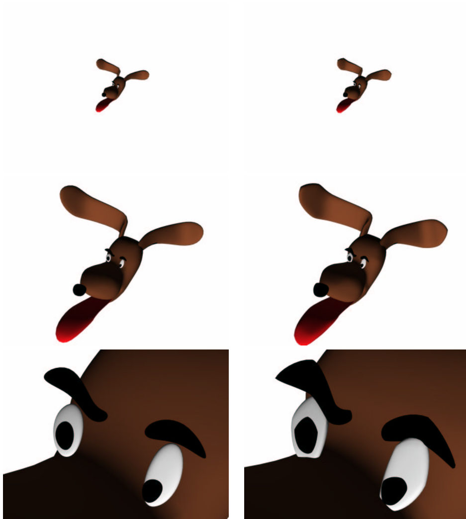
Catmull-Clark
