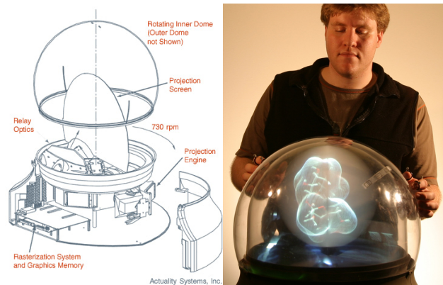
Figure 2. Volumetric display
