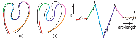
Figure 9: Equal weights for all sample points (a), and only weighting the end-points (b), result in different rigid transforms for the same composite curve segmentation on the right.
